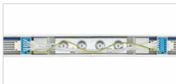
Very stable coupling between the trunking rails for long suspension distances of up to 4.6 m
